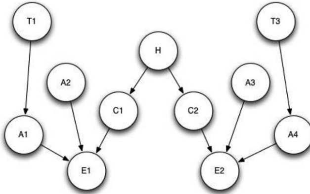
Figure 2. Bayesian network representation of an ideal robustness argument.
