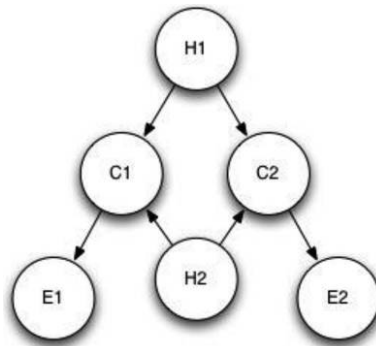
Figure 6. H1 does not d-separate E1 and E2 because of the presence of the alternate hypothesis H2 (and therefore an alternate trail between E1 and E2).
