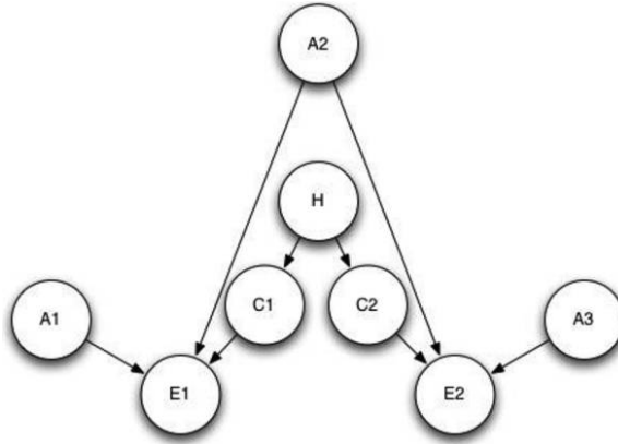
Figure 3. Auxiliary assumption (A2) influences both modes of evidence, and so H no longer d-separates E1 and E2.
