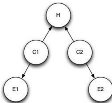
Figure 5. H does not d-separate E1 and E2 , because, even though it lies on the only trail between E1 and E2 , it is a collider.
