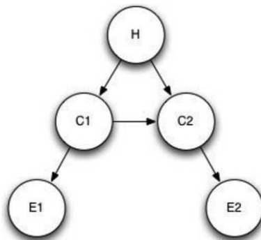
Figure 4. H no longer d-separates E1 and E2 because there is a dependency between C1 and C2 (and thereby between E1 and E2 ), even if we conditionalize on H .
