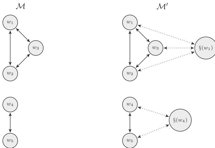
Figure 1. Extending a Kripke model.
