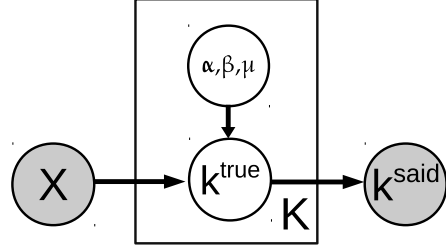
Figure 4: The Rational Observer observes a color patch, x . The applicability of each label ( k^{true} ) is based upon the label parameters ( \alpha, \beta, \mu ) and x . The label ( k^{said} ) is sampled proportional to the applicability and a background weight: how often a label is said when it applies.
