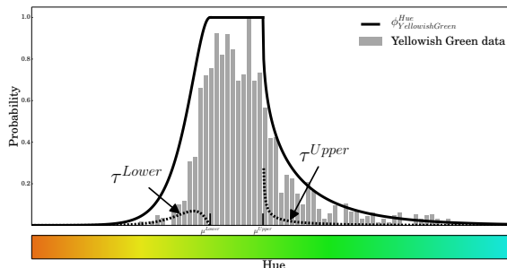
Figure 3: The LUX model for “yellowish green” on the Hue axis plotted against the scaled histogram of the responses in the data. The \phi curve represents the likelihood of “yellowish green” for different Hue values. The \tau curves represent possible boundaries.
