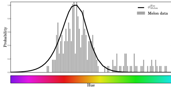
Figure 5: For the Hue dimension, the data for “melon” is plotted against the LUX model’s \phi curve.
