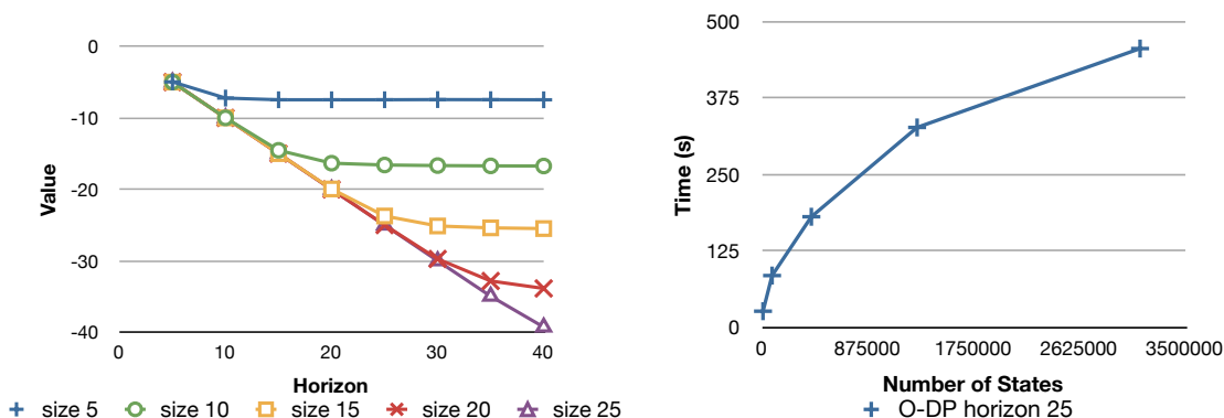
Figure 9: Value and time results for O-DP in the two-agent NAMO problem for various size grids (where size is the length of a single side)
