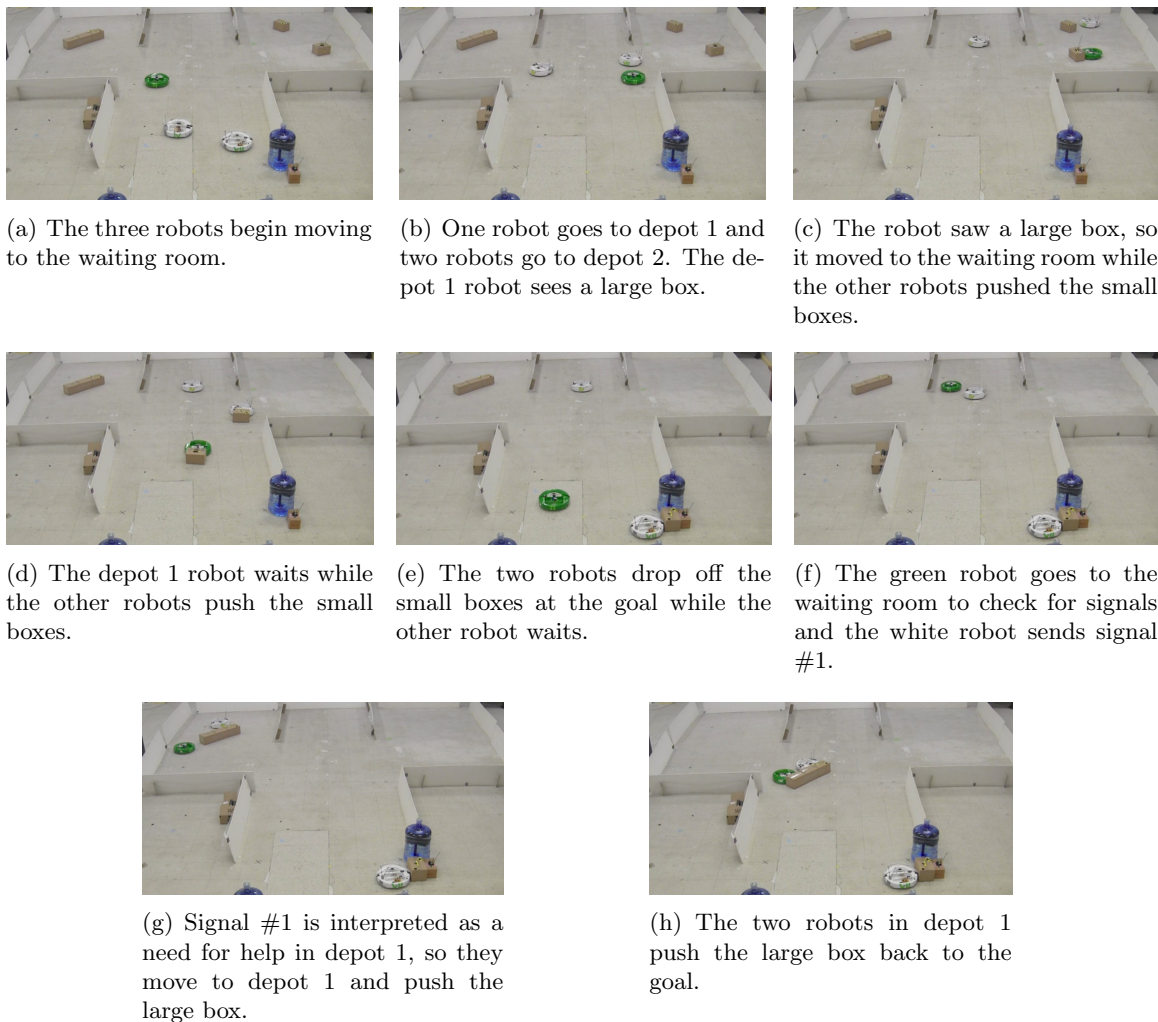
Figure 13: Scenario 2 (limited communication).
