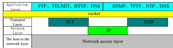
Figure 5. TCP/IP Architecture
