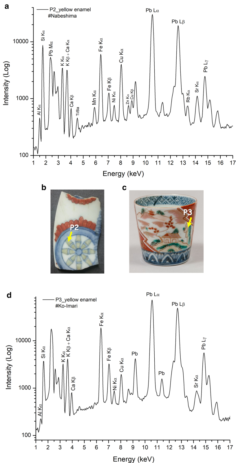
Fig. 8 a, b Nabeshima Shard (1690–1730) and Pb–Fe yellow enamel XRF spectrum; c, d Ko-Imari cup (1770–1790) and Pb–Fe yellow enamel XRF spectrum
