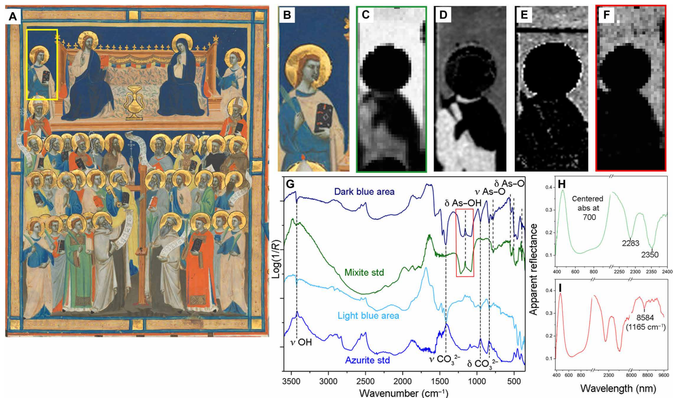
Fig. 5. Christ and the Virgin Enthroned with Forty Saints : Identification and mapping of azurite and mixite in blue areas. (A) Color image of the Master of the Dominican Effigies' Christ and the Virgin Enthroned with Forty Saints (ca. 1340), Rosenwald Collection, National Gallery of Art. (B) Color detail studied. (C) Map of azurite obtained from the reflectance spectrum (H). (D) Elemental map of zinc (K \alpha ). (E) Elemental map of As (K \beta ). (F) Map of the As—OH reflectance feature attributed to mixite and the spectral features of azurite in visible and NIR (I). (G) Mid-IR reflectance spectra of the dark blue and light blue areas, in addition to mixite and azurite standards.
