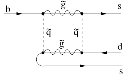
Figure 11. MSSM squark-gaugino box diagram for b \rightarrow s s \bar{d} .
