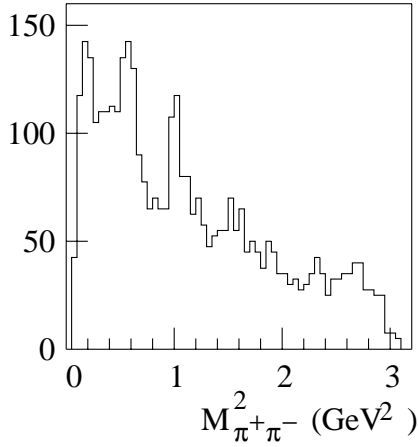
Figure 9. M_{\pi^+\pi^-}^2 distribution for D^+ \rightarrow \pi^-\pi^+\pi^+ .
