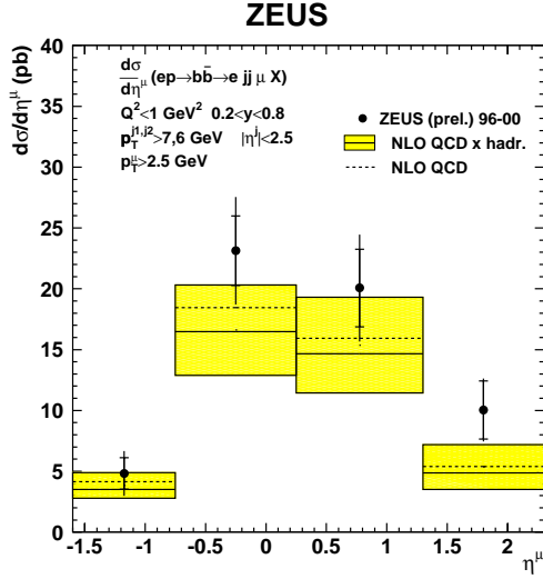
Figure 1. Differential cross section of beauty photoproduction as a function of the muon pseudorapidity compared with NLO QCD calculations.
