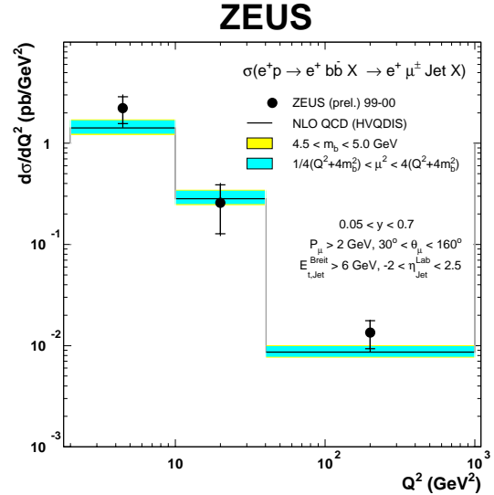
Figure 2. Differential beauty cross section as a function of Q^2 compared with the NLO QCD calculations.
