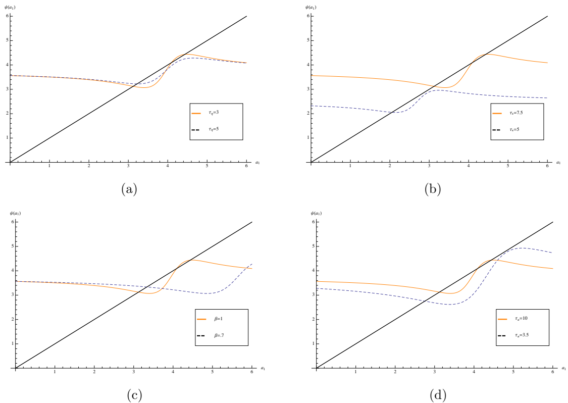
Figure 2: Comparative statics. We plot the best response (22) for the parameters' value of Figure 1 (in orange) and show the effect of a change in the values of \tau_\eta , \tau_\varepsilon , \beta , and \tau_u (dashed, blue curve). In panel (a) we increase public signal precision to \tau_\eta = 5 ; in panel (b) we decrease private signal precision to \tau_\varepsilon = 5 ; in panel (c) we decrease liquidity traders' persistence to \beta = .7 , and in panel (d) we decrease the precision of liquidity traders' demand to \tau_u = 3.5 .
