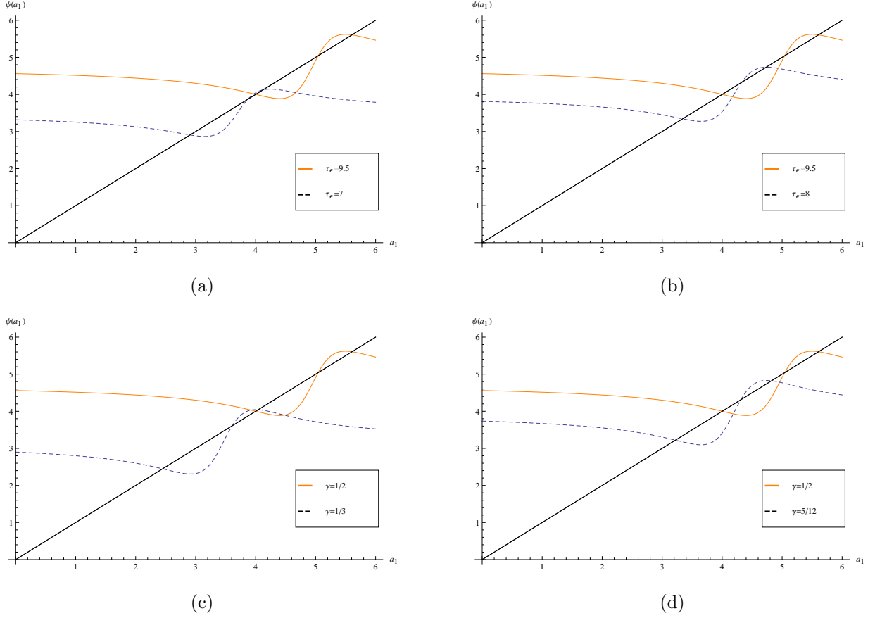
Figure 6: Adjustment to a shock when the HIE is stable. We plot the best response (22) for \tau_v = \tau_u = 10 , \gamma = 1/2 , \tau_\eta = 3 , \beta = 1 , and \tau_\varepsilon = 9.5 (orange). In panel (a) and (b) we analyze the effect of a reduction in the precision of the private signal to \tau_\varepsilon = 7 (dashed best response, panel (a)) and \tau_\varepsilon = 8 (dashed best response, panel (b)). In panel (c) and (d) we analyze the effect of a reduction in risk tolerance to \gamma = 1/3 (dashed best response, panel (c)) and \gamma = 5/12 (dashed best response, panel (d)).
