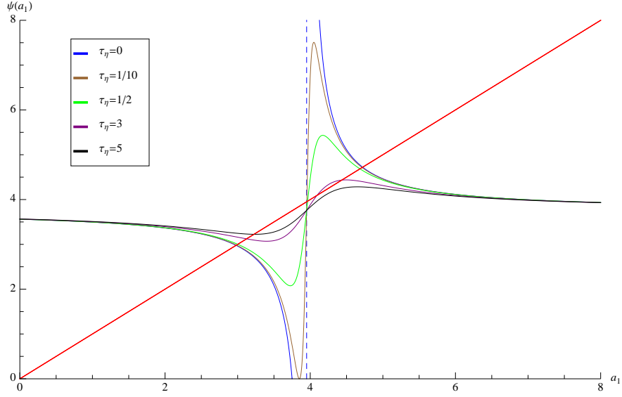
Figure 3: The best-response mapping (22) when the public signal's precision ranges within the set \{0, 1/10, 1/2, 3, 5\} . The other parameter values are \beta = 1 , \gamma = 1/2 , \tau_u = \tau_v = 10 , \tau_\varepsilon = 7.5 , and \tau_\eta = 0 . When \tau_\eta = 0 , note that \psi(\cdot, \tau_\eta) diverges at the point \hat{a}_1 \equiv (1 + \gamma\tau_u a_2)/(\gamma\beta\tau_u) and the IIE disappears. For \tau_\eta > 0 , we have \psi(\hat{a}_1, .1) = 3.75864 , \psi(\hat{a}_1, .5) = 3.75862 , \psi(\hat{a}_1, 3) = 3.7585 , and \psi(\hat{a}_1, 5) = 3.7584 .
