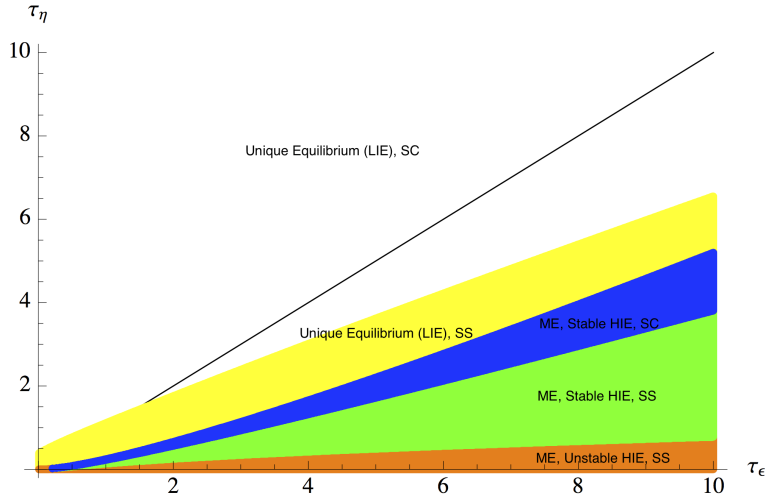
Figure 4: The equilibrium set for \beta = 1 , \gamma = 1/2 , \tau_u = \tau_v = 10 , \tau_\eta \in \{0, .01, \dots, 10\} , and \tau_\varepsilon \in \{.01, .02, \dots, 10\} . The black line denotes the set \tau_\eta = \tau_\varepsilon . For values of (\tau_\varepsilon, \beta) in the white and yellow regions, the equilibrium is unique, whereas multiple equilibria (ME) obtain when (\tau_\varepsilon, \beta) are in the other regions, where the HIE can be stable or unstable depending on the difference between \tau_\eta and \tau_\varepsilon .
