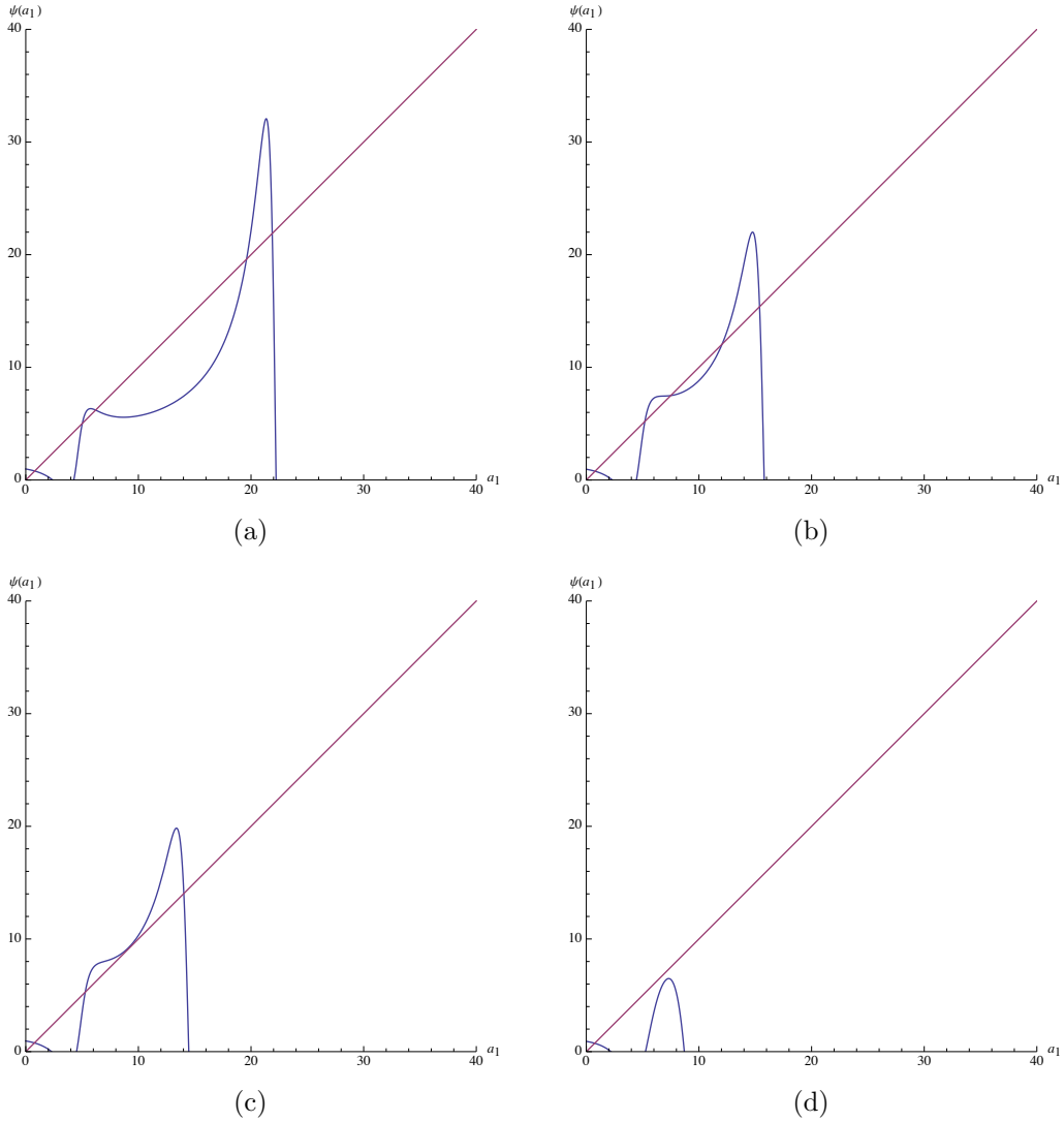
Figure 8: The best response mapping in the model with residual uncertainty. Parameters' values are \tau_u = \tau_v = 1 , \tau_\varepsilon = 4 , \tau_\eta = 2/3 , \gamma = 1 , and \beta = 1 . When \tau_\delta \in \{75, 100\} , five equilibria obtain, only two of which are stable (respectively, panel (b), and (a)). When \tau_\delta = 70 , only the LIE is stable (panel (c)). When \tau_\delta = 40 , only the LIE survives (panel (d)).
