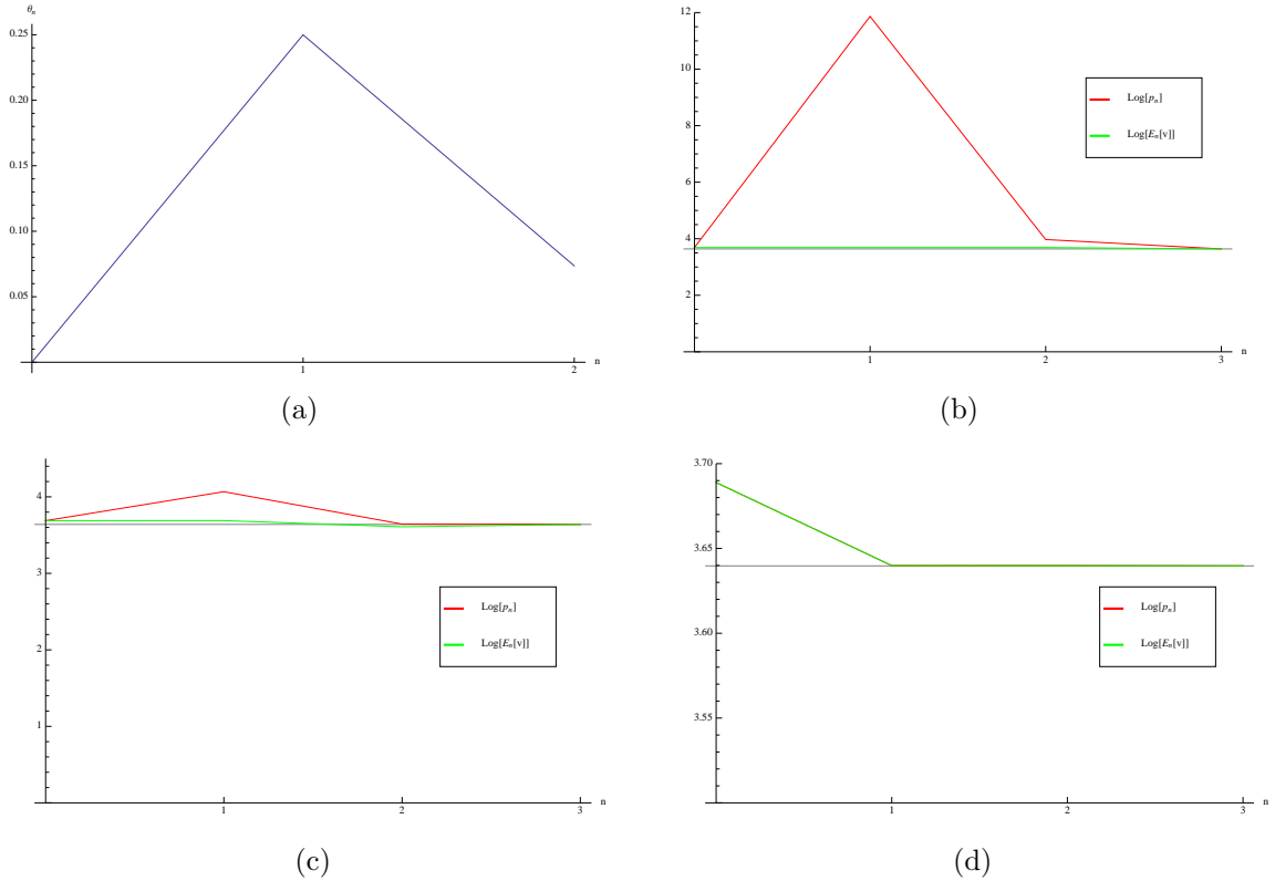
Figure 5: Liquidity traders' demand (panel (a)) and the path of prices (red) and semi-strong efficient prices (green) along the equilibrium with no private information, the LIE, and the HIE (respectively, panels (b), (c), and (d)). Parameter values are as follows: \bar{v} = 40 , \tau_v = .01 , \tau_u = .1 , \tau_\varepsilon = 1 , \gamma = 1/2 , \tau_\eta = .001862 , and \beta = 1/2 .
