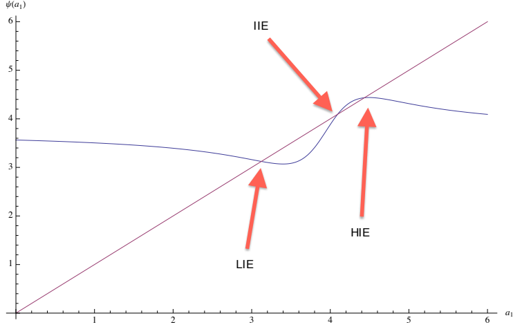
Figure 1: The best-response mapping (22) for \beta = 1 , \gamma = 1/2 , \tau_u = \tau_v = 10 , \tau_\eta = 3 , and \tau_\varepsilon = 7.5 .
