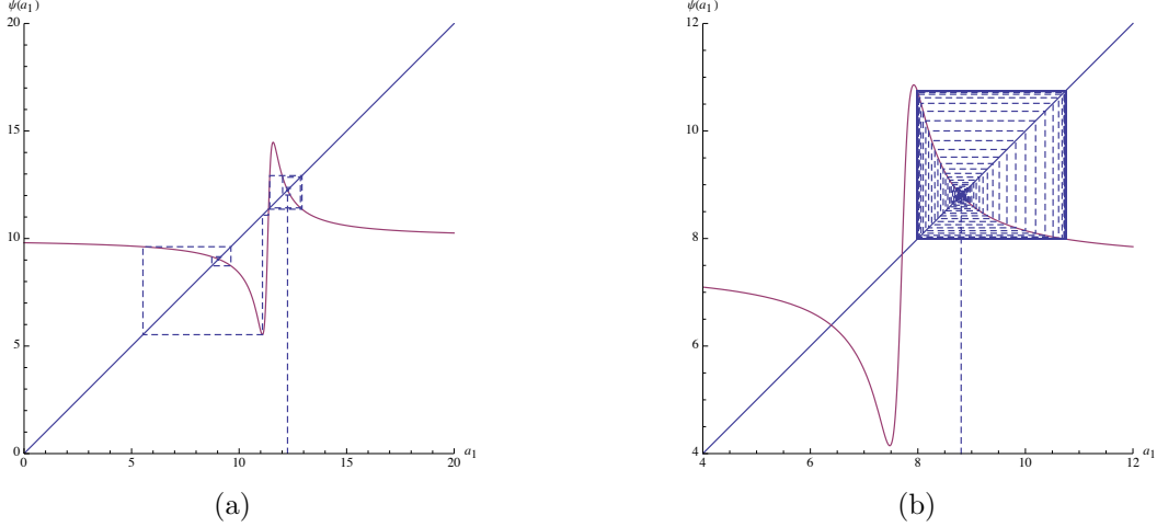
Figure 7: Adjustment to a shock when the HIE is unstable. In panel (a) we plot the best response (22) for \tau_v = \tau_u = 10 , \tau_\varepsilon = 20 , \gamma = 1/2 , \tau_\eta = 1/2 , and \beta = .9 . With these parameter values, the LIE and HIE are respectively a_1^* = 9.04 , and a_1^{***} = 12.25 , and the slope of the best response at these two points is given by \psi'(a_1^*) = -.41 and \psi'(a_1^{***}) = -2.12 . In panel (b) we plot the best response (22) for \tau_v = \tau_u = 10 , \tau_\varepsilon = 15 , \gamma = 1/2 , \tau_\eta = 1/2 , and \beta = 1 . With these parameter values, the LIE and HIE are respectively a_1^* = 6.64 , and a_1^{***} = 9.37 , and the slope of the best response at these two points is given by \psi'(a_1^*) = -.43 and \psi'(a_1^{***}) = -1.9 .
