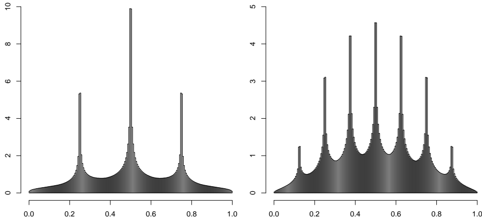
FIGURE 1: Normalized histograms each based on 10^8 simulations, with N = 3 and initial points \frac{1}{4}, \frac{1}{2}, \frac{3}{4} (left) and N = 7 and initial points \frac{k}{8}, k \in \{1, \dots, 7\} (right).
