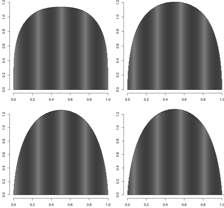
FIGURE 2: Normalized histograms for 10^8 simulations with random i.i.d. uniform initial conditions, with ( top row ) N = 3, 10 and ( bottom row ) N = 50, 100 .
