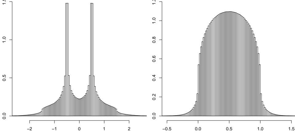
FIGURE 4: Normalized histograms based on 10^8 simulations of the modified N = 3 model with fixed \{-1/2, 1/2, 100\} initial condition ( left ) and i.i.d. U[0, 1] initial condition ( right ).
