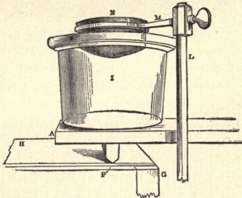
FIG. II. CROOKES' APPARATUS.
