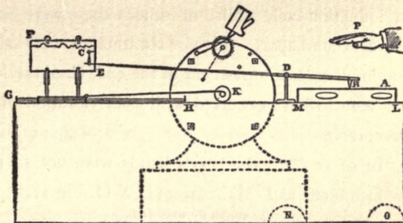
FIG. 17. SECTION OF APPARATUS IN FIG. 16.
