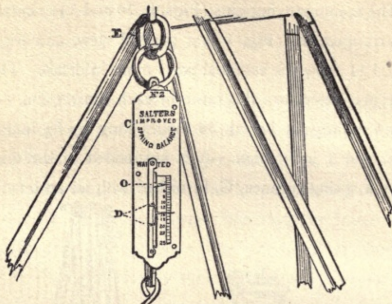
FIG. 10. CROOKES' APPARATUS.
