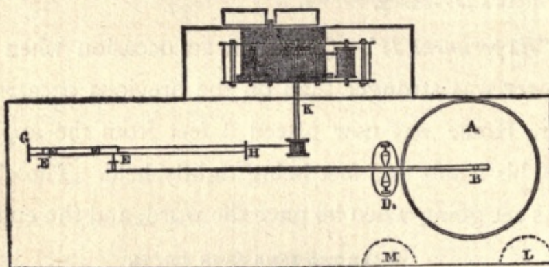
FIG. 16. SECOND CROOKES' APPARATUS.
